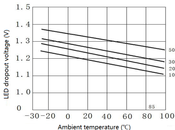
● LED dropout voltage vs Ambient Temperature
