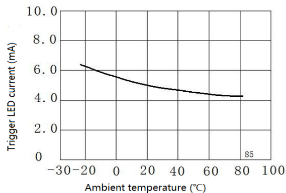
● Trigger LED current vs Ambient Temperature
