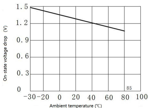
● On-state voltage drop vs Ambient Temperature
